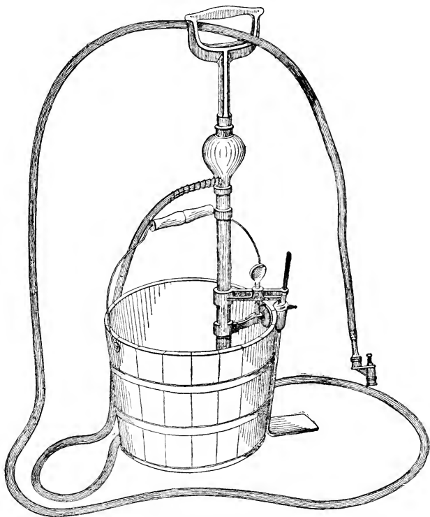
FIG. 5.—Pail spraying pump for small herds.
